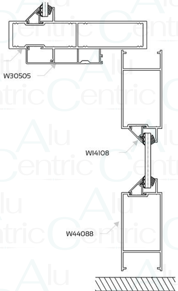
SECTION B-B
