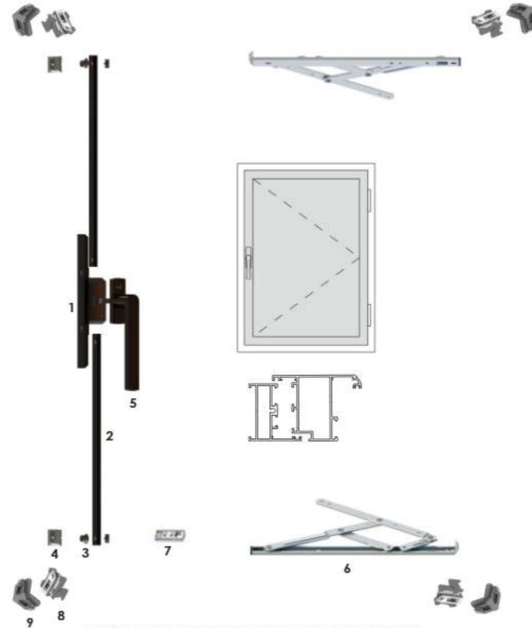
CASEMENT WINDOW HARDWARE CONFIGURATION :
