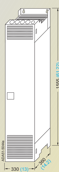
Inverter frame size FX
