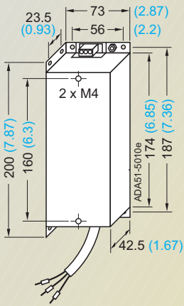
Filter for frame size A
