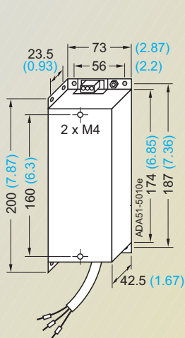
Filter for frame size A
