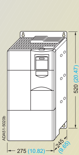
Inverter frame size D
