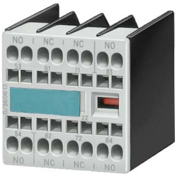
AUXILIARY SWITCH BLOCK, 11E (1NC), DIN EN50012, CAGE CLAMP CONNECTION, FOR CONTACTORS FOR SWITCHING MOTORS, 4-POLE
