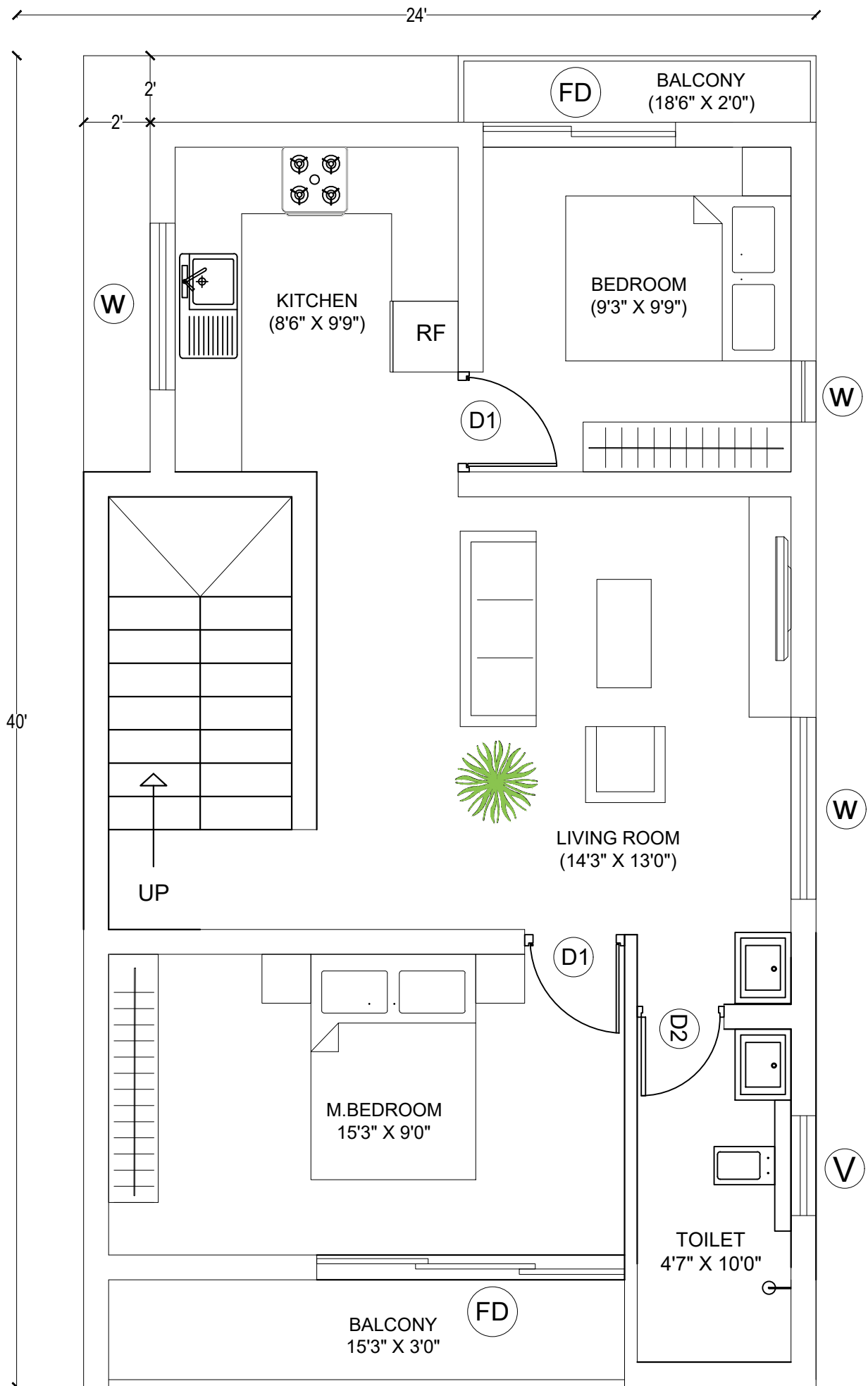
FIRST FLOOR - 837SQFT + HEADROOM - 100SQFT
