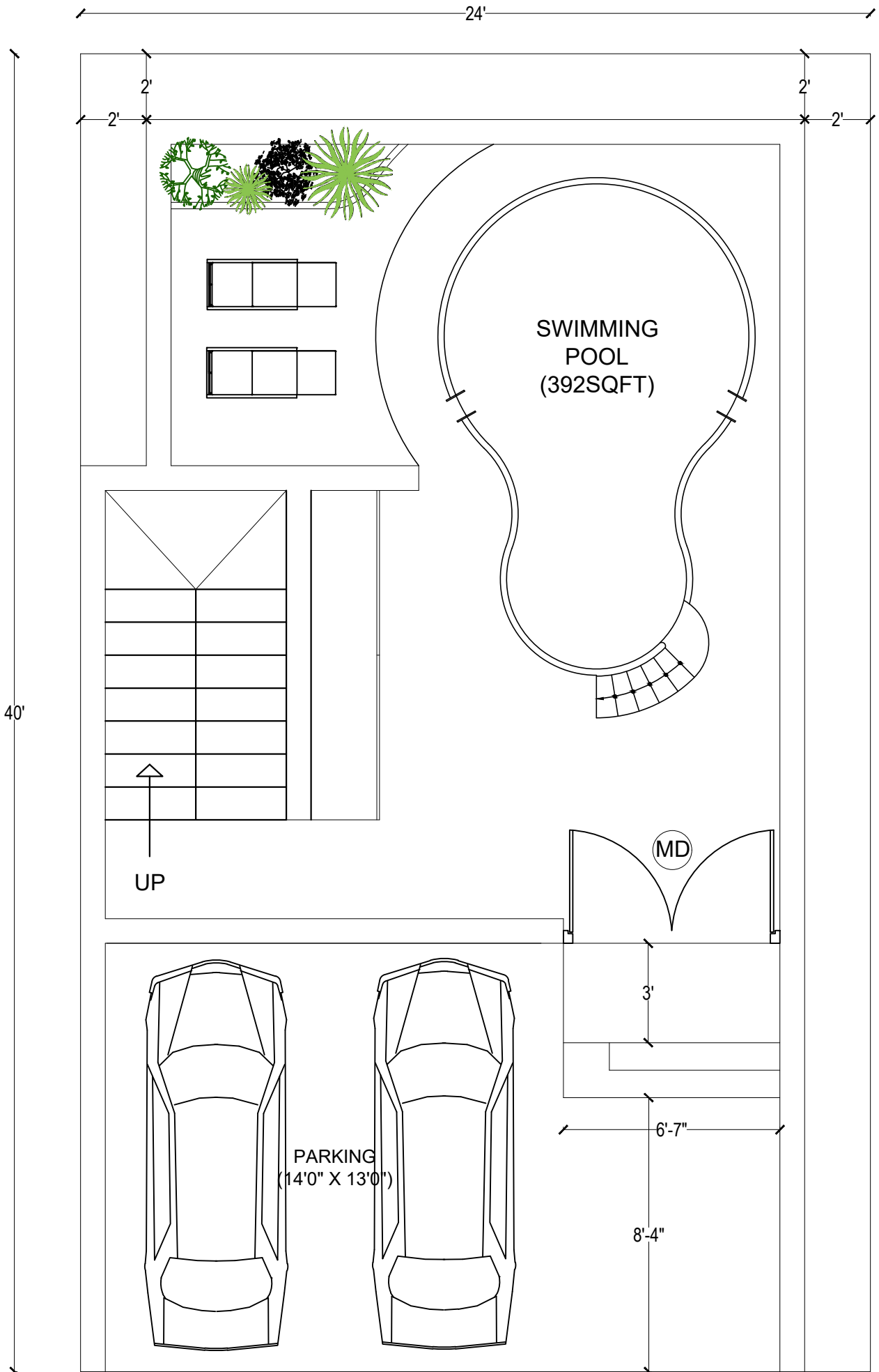
GROUND FLOOR 814SQFT
