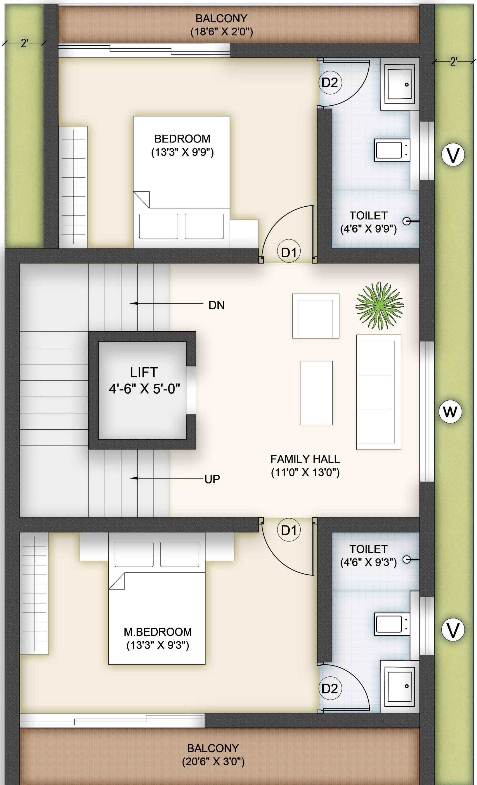
SECOND FLOOR 854SQFT
