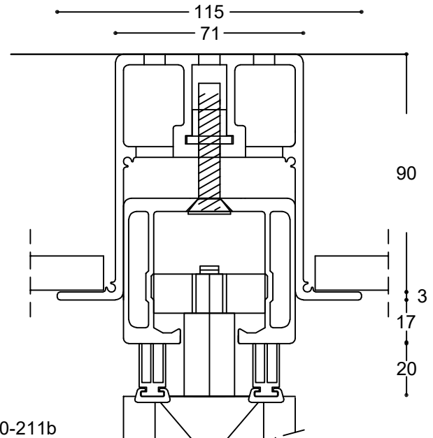
Justerbar styreskinne - Rw 31-46 db - type UPL-TP
