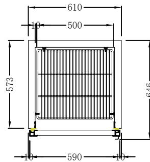
PLAN (顶视)
