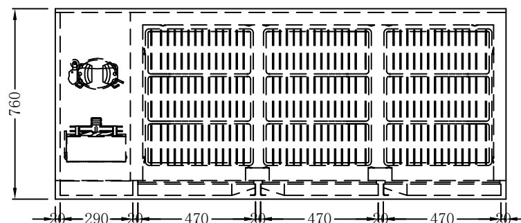
PLAN (顶视)
