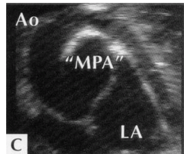
Type 1-2
