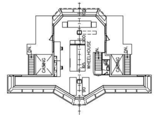
BRIDGE DECK
