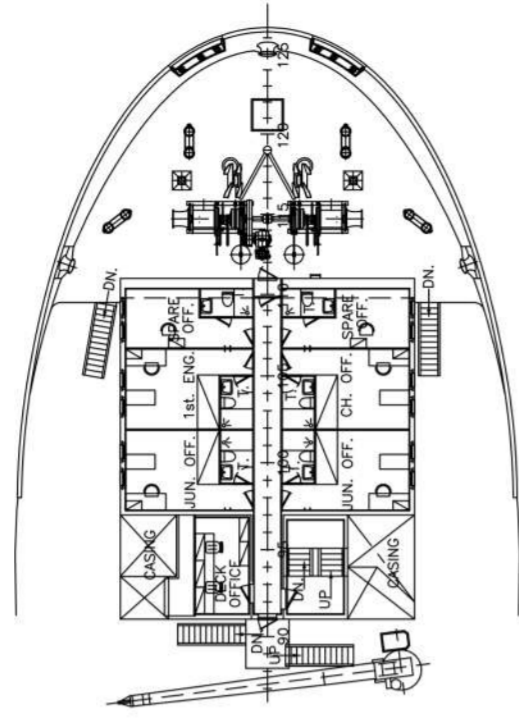
B-DECK
